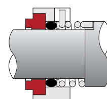
PT01FE/Q22X/03_ (Ext LH parallel spring with pin)
